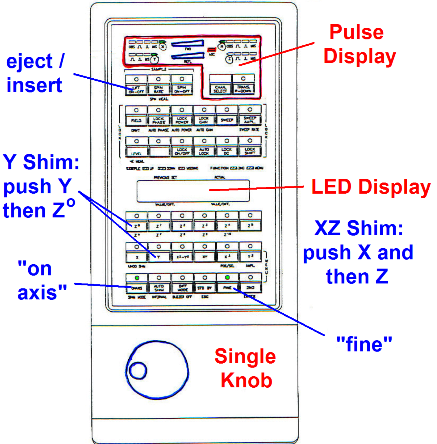
Figure 4: Layout of BSMS-Keyboard
