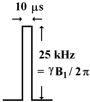
Hard 90° Pulse
